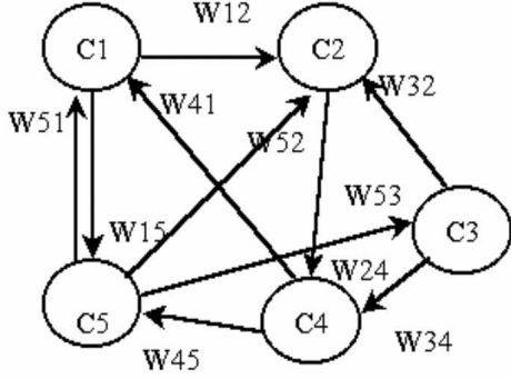
Fig. 1. A simple FCM with 5 concepts and 10 weights.
