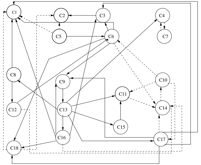
Fig. 2. The FCM for the Eco-Industrial Park.
